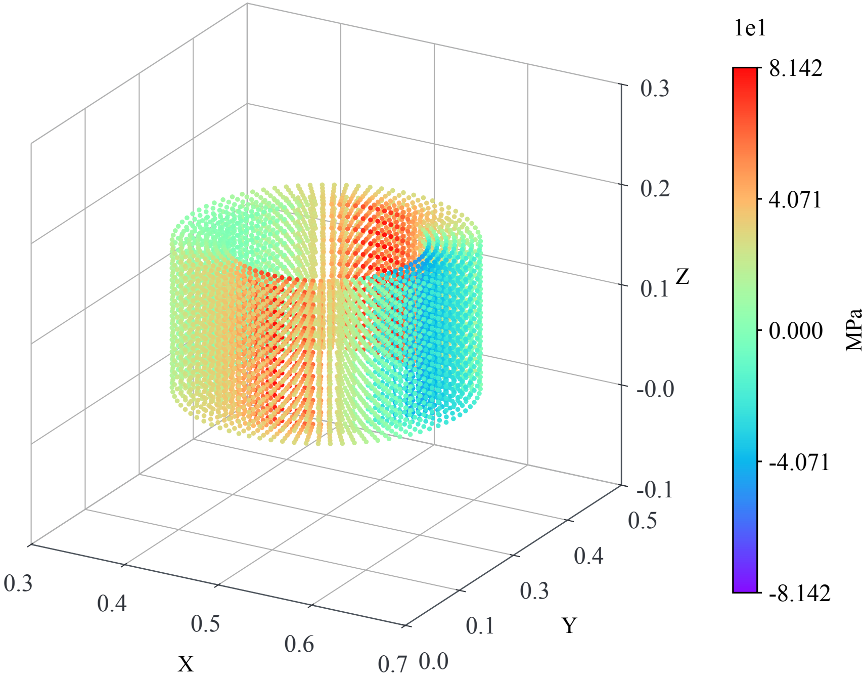
\sigma_{xx} Prediction
