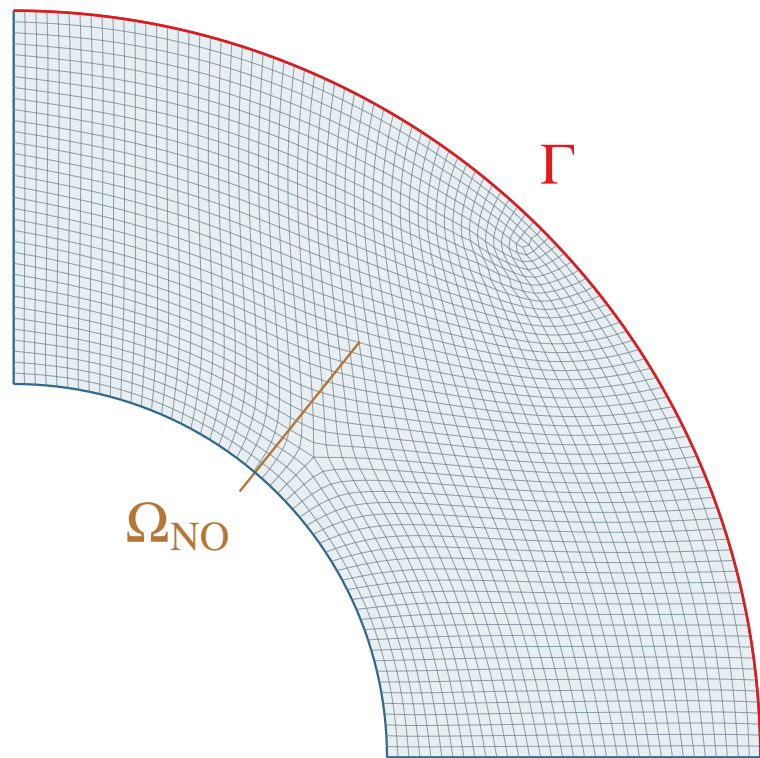
(a) QUAD4 mesh
