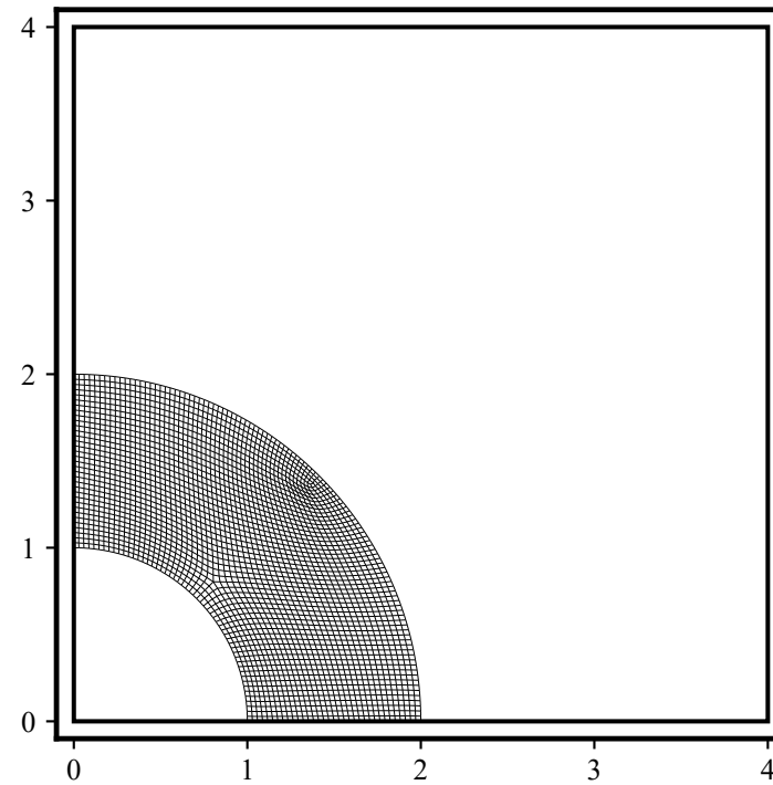
Subdomain Mesh
