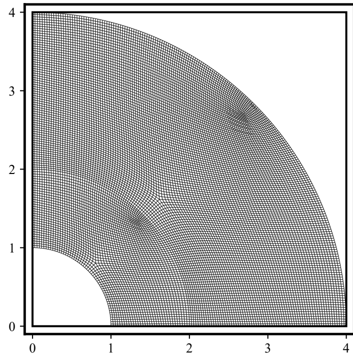
Full Domain Mesh
