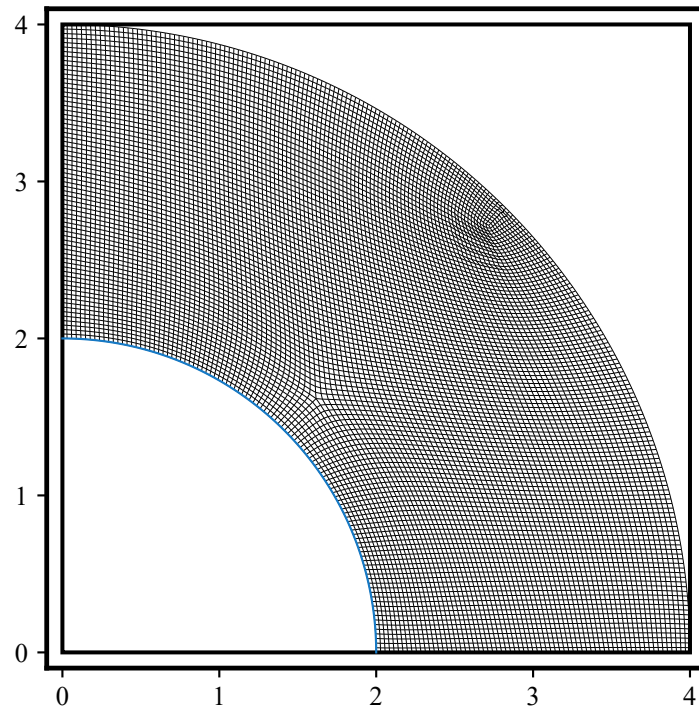
Outer Domain Mesh
